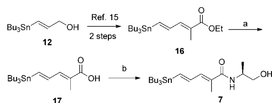
Scheme 4. Synthesis of right-hand fragment 7 . Reagents and conditions: a) TMSOK, THF, RT; b) 11 , PyBroP, i\text{Pr}_2\text{NEt} , \text{CH}_2\text{Cl}_2 , 0^\circ\text{C} to RT, 94 % (2 steps). THF = tetrahydrofuran, TMS = trimethylsilyl, PyBroP = bromotripyrrolidinophosphonium hexafluorophosphate.
