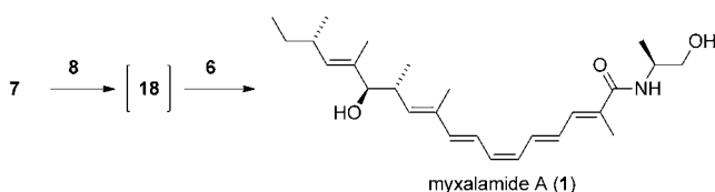
Scheme 5. Completion of the total synthesis of (–)-myxalamide A by a one-pot Stille/Suzuki–Miyaura coupling reaction. Reagents and conditions: 8 , [\text{Pd}_2(\text{dba})_3 \cdot \text{CHCl}_3] , JohnPhos, \text{CH}_3\text{CN} , DMF, -10^\circ\text{C} , 24 h; then 6 , 1 M aq. NaOH, [\text{Pd}_2(\text{dba})_3 \cdot \text{CHCl}_3] , 0^\circ\text{C} to RT, 22 h, 59%.
